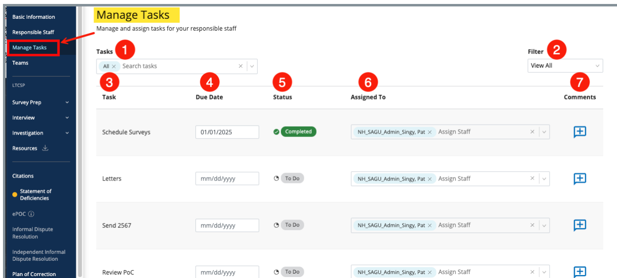
Figure 45: Manage Tasks
