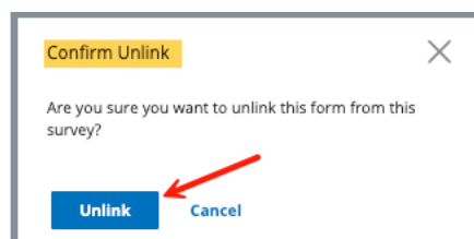
Figure 140: Confirm Unlink
