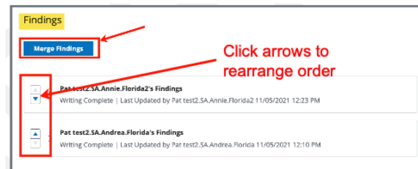
Figure 97: Findings
