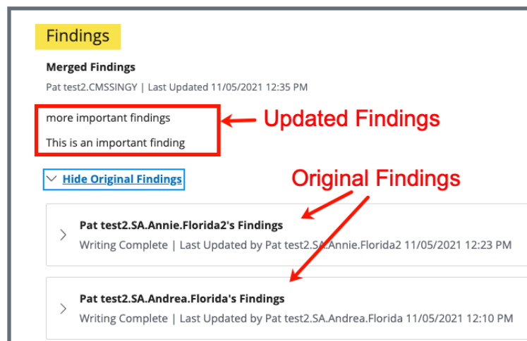
Figure 100: Findings
