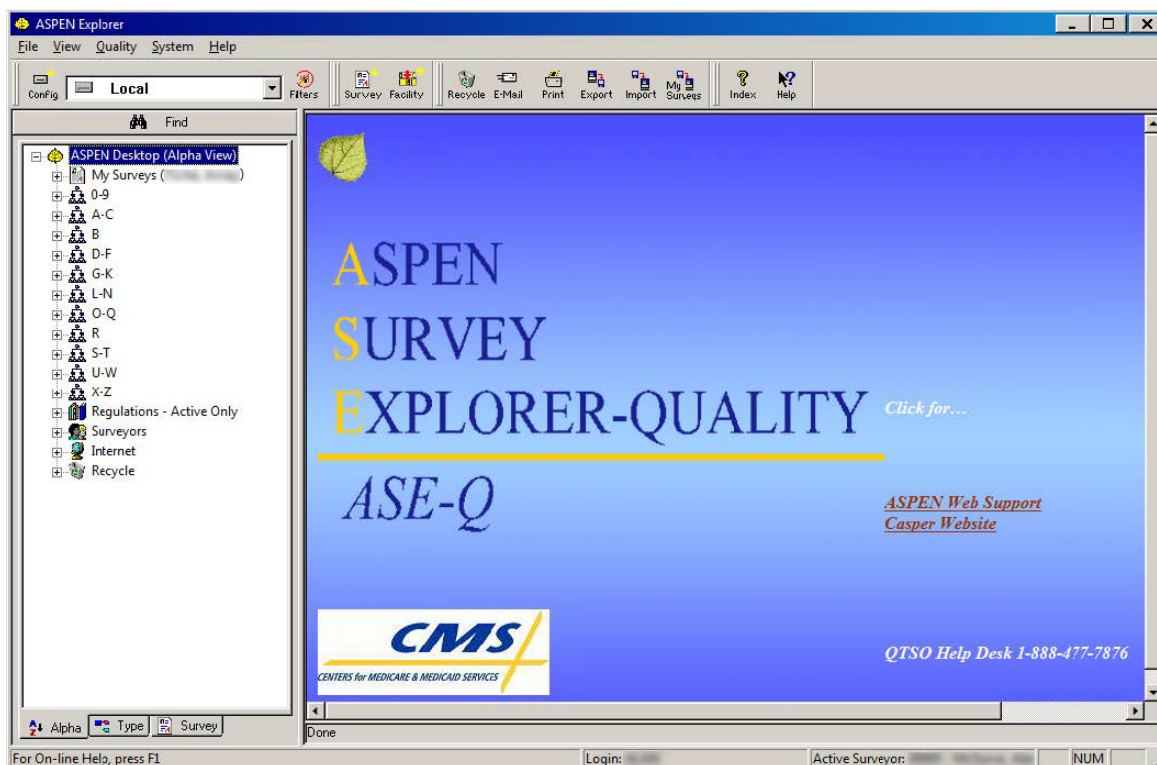
Figure 11: Tree view
