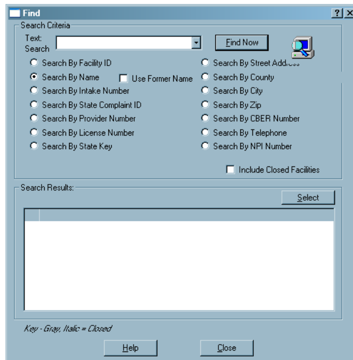
Figure 153: Find window
